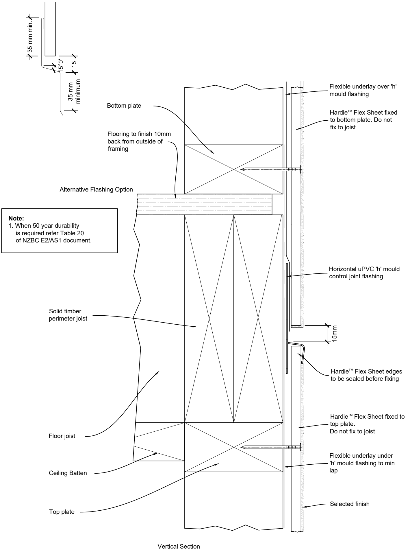
fig13 jhl_flex_d_junc_join-hrzn.dwg
